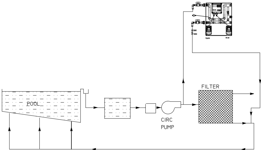
Typical Installation Schematic
