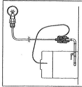
Fig. 8: Flooded suction mounting
