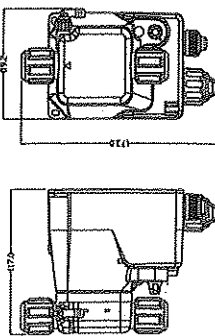
Fig. 4: Overall dimensions of pump
